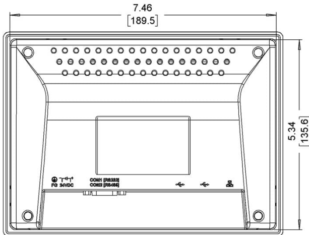
Rear View
