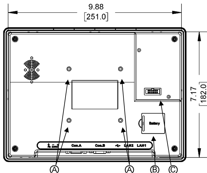
Rear View
