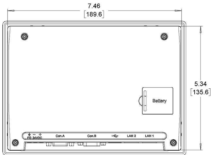
Rear View
