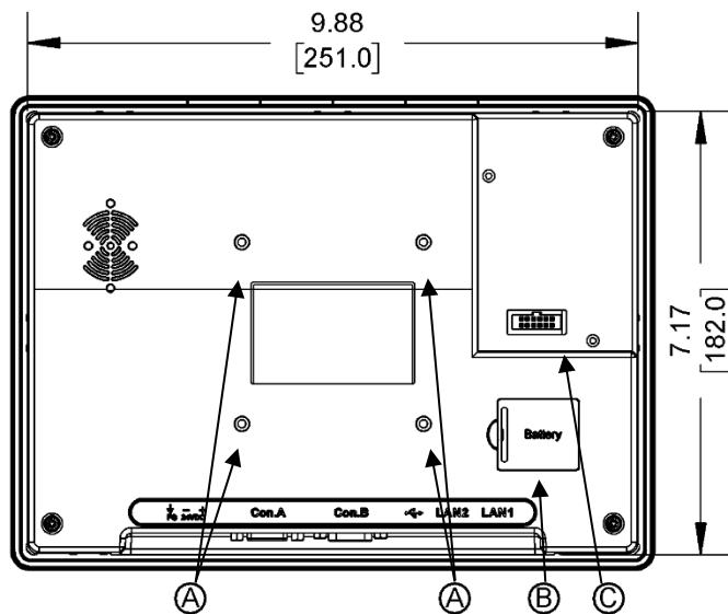
Rear View
